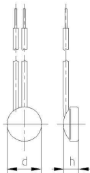
Diameter d 9,0 mm Installation height h from 4,5 mm
